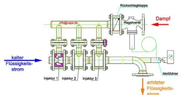
Heisswasserstation
